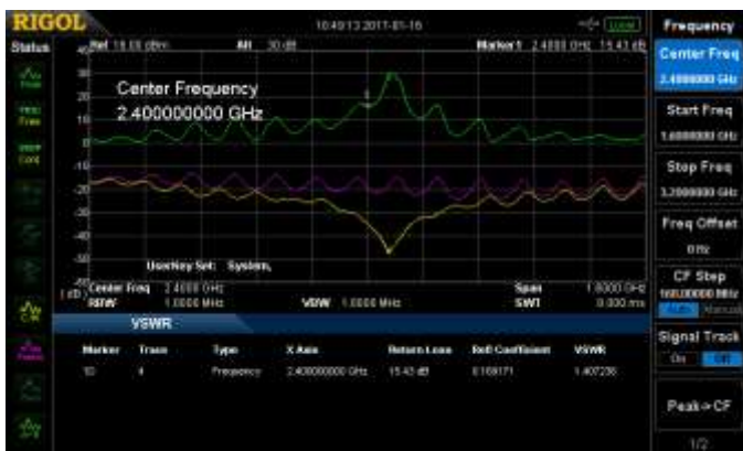
Figure 2: The image shows a VSWR test being performed on an antenna that is meant to operate at 2.4 GHz and has a VSWR of 1.17.
