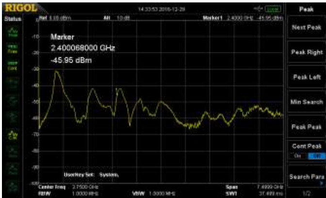
Figure 1: A bandwidth test being performed on two matched antennas that are rated for the 2.4GHz bandwidth.
